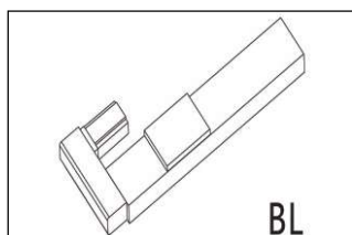
YR-MGWS75F Primary Configuration/Parameters Adaptation Motor 57 stepping motor, 100W/200W/400W Servo Motor Linear Guideway MGR12*1 MGW12H*1 Ball Screw Φ 16—C7 Repeatable Positioning Accuracy ( mm ) ± 0.02 Lead Screw ( mm ) 5 10 16 20 Max Speed ( mm/s ) 250 500 800 1000 Maximum Handling Weight ( Kg ) Horizontal 30 25 20 15 Vertical 30 25 20 15 Stroke Range ( mm ) 100—800
